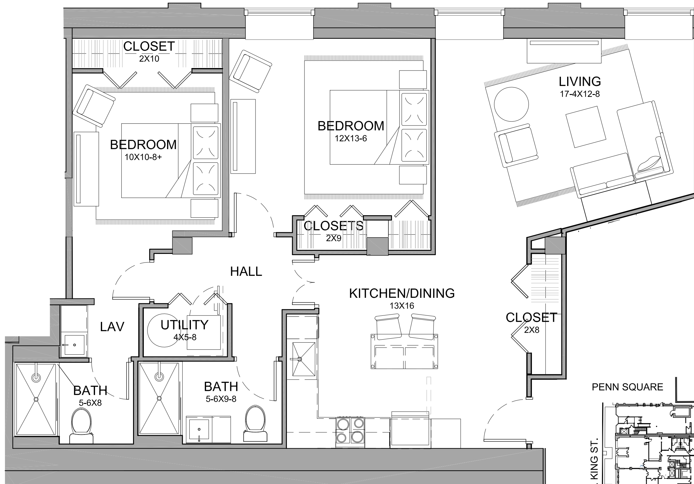
1 1ST FLOOR - APARTMENT 106 1/4" = 1'-0" @11X17 1102 SF LEASABLE
